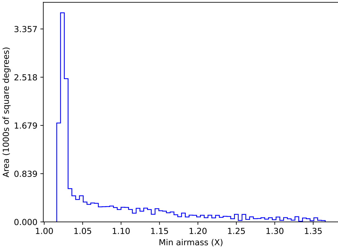
ddf_acor_sf15_lsf20_lsr20_v3.4_10yrs WFD all bands: Min airmass
