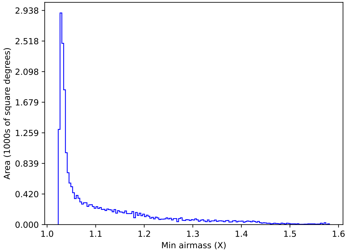
ddf_acor_sf15_lsf20_lsr20_v3.4_10yrs All sky y band: Min airmass
