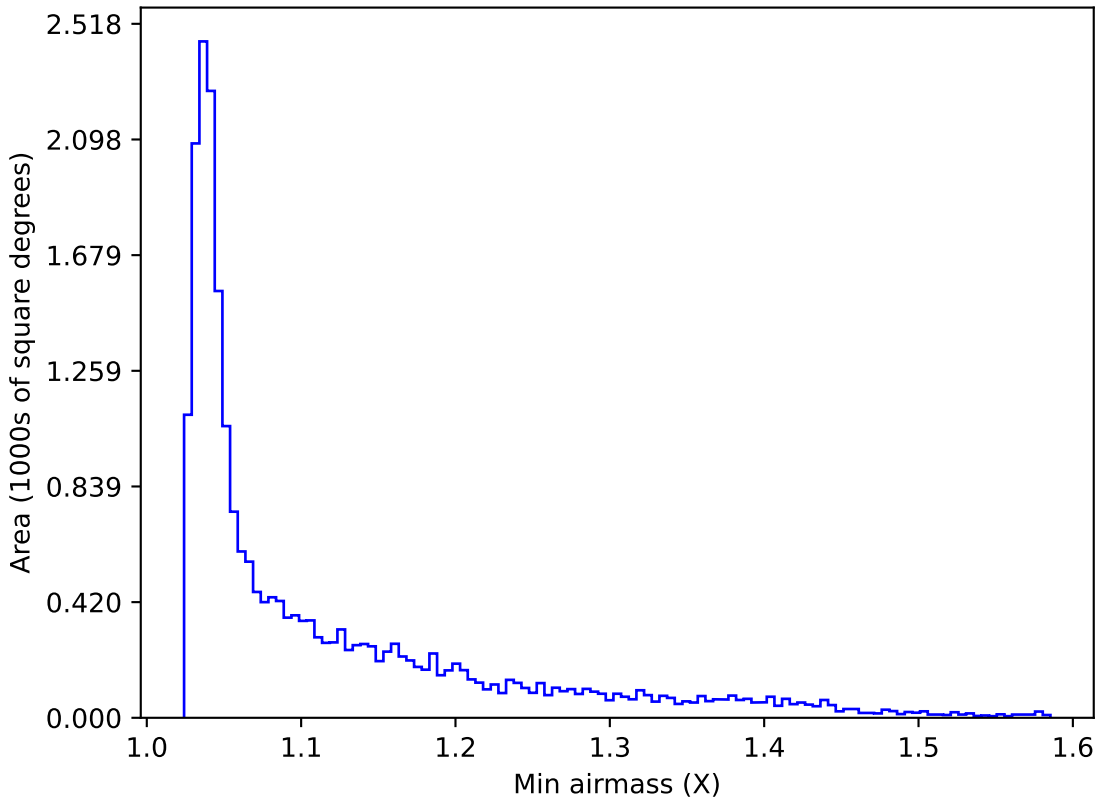
ddf_acor_sf15_lsf20_lsr20_v3.4_10yrs All sky u band: Min airmass
