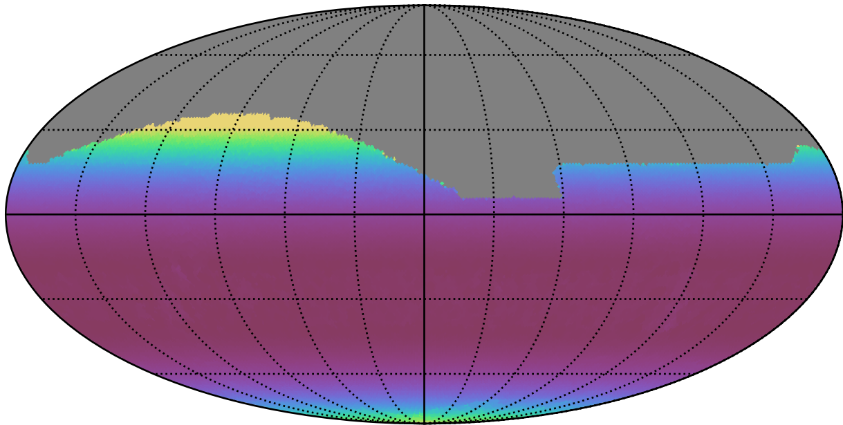
ddf_acor_sf15_lsf20_lsr20_v3.4_10yrs All sky r band: Min airmass
