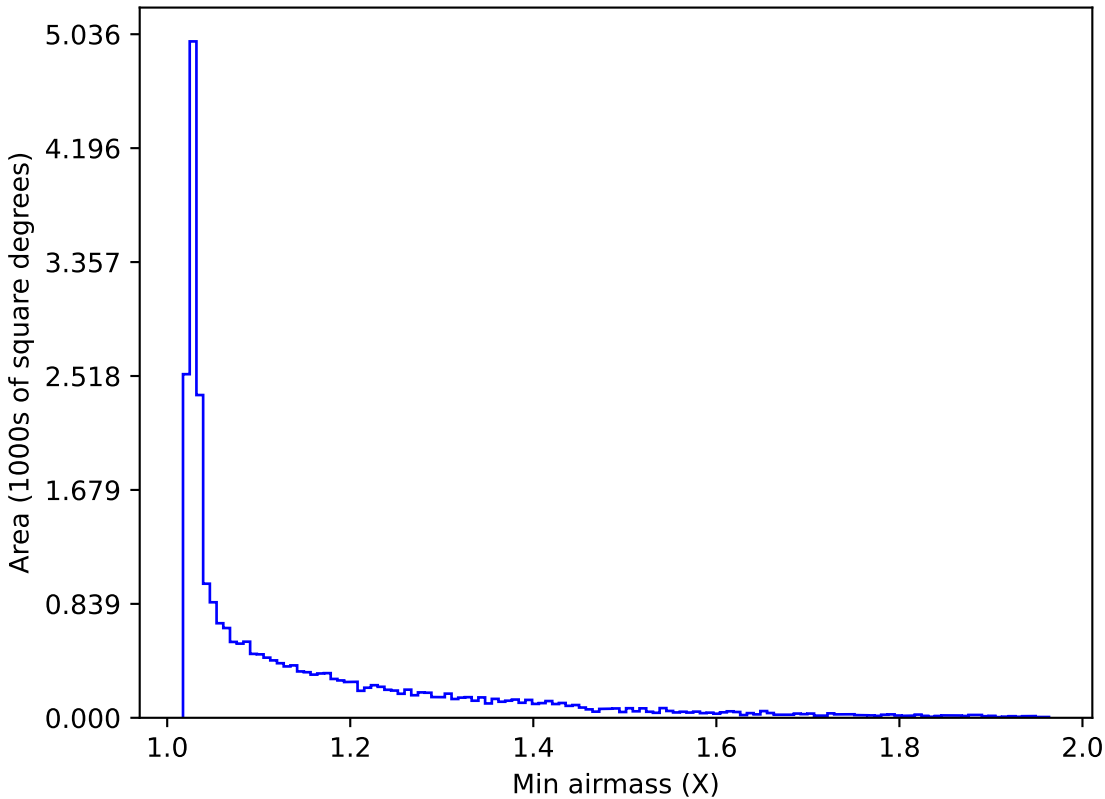
ddf_acor_sf15_lsf20_lsr20_v3.4_10yrs All sky r band: Min airmass
