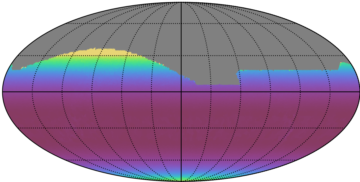
ddf_acor_sf15_lsf20_lsr20_v3.4_10yrs All sky i band: Min airmass
