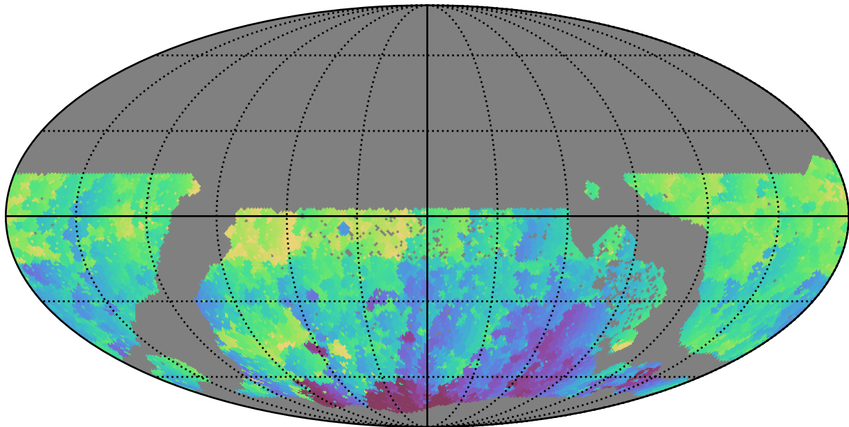
ddf_acor_sf15_lsf20_lsr20_v3.4_10yrs WFD u band: Min HA
