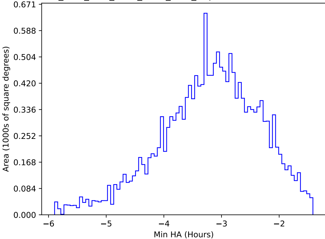
ddf_acor_sf15_lsf20_lsr20_v3.4_10yrs WFD u band: Min HA
