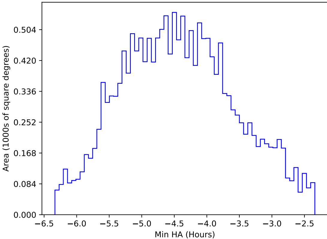
ddf_acor_sf15_lsf20_lsr20_v3.4_10yrs WFD r band: Min HA
