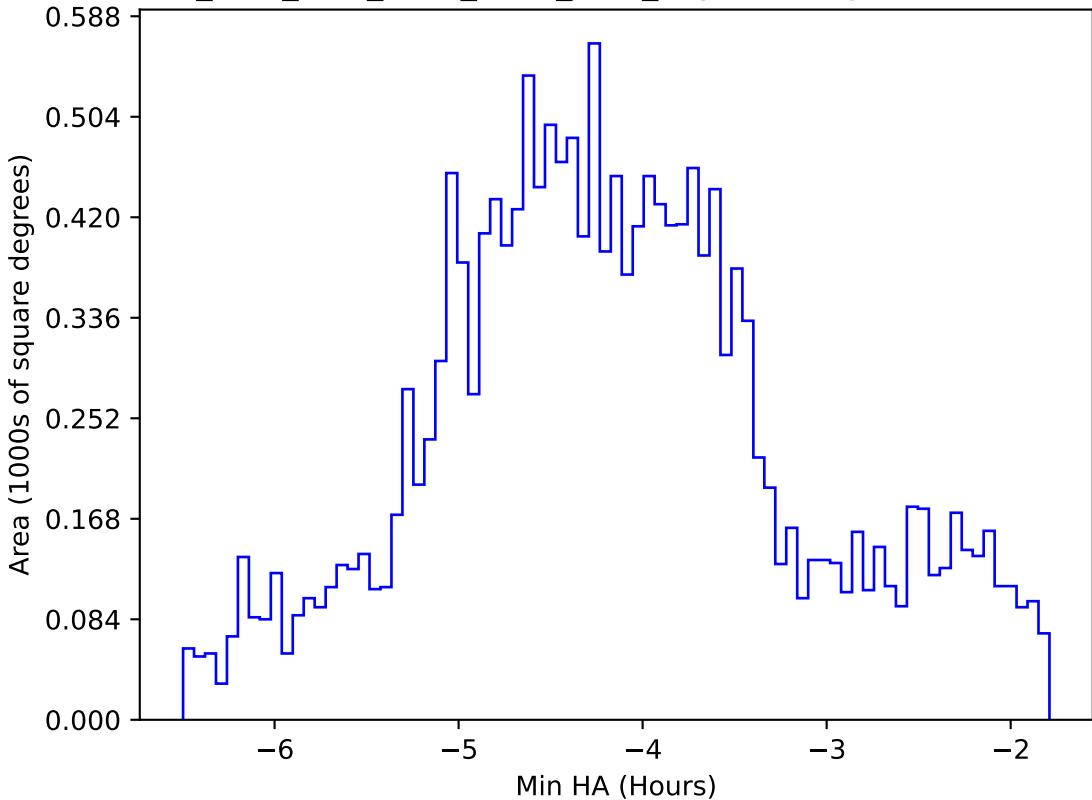
ddf_acor_sf15_lsf20_lsr20_v3.4_10yrs WFD g band: Min HA
