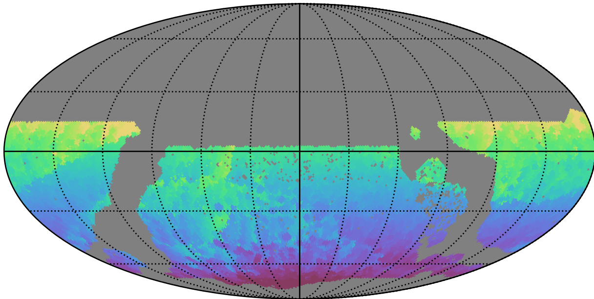
ddf_acor_sf15_lsf20_lsr20_v3.4_10yrs WFD all bands: Min HA
