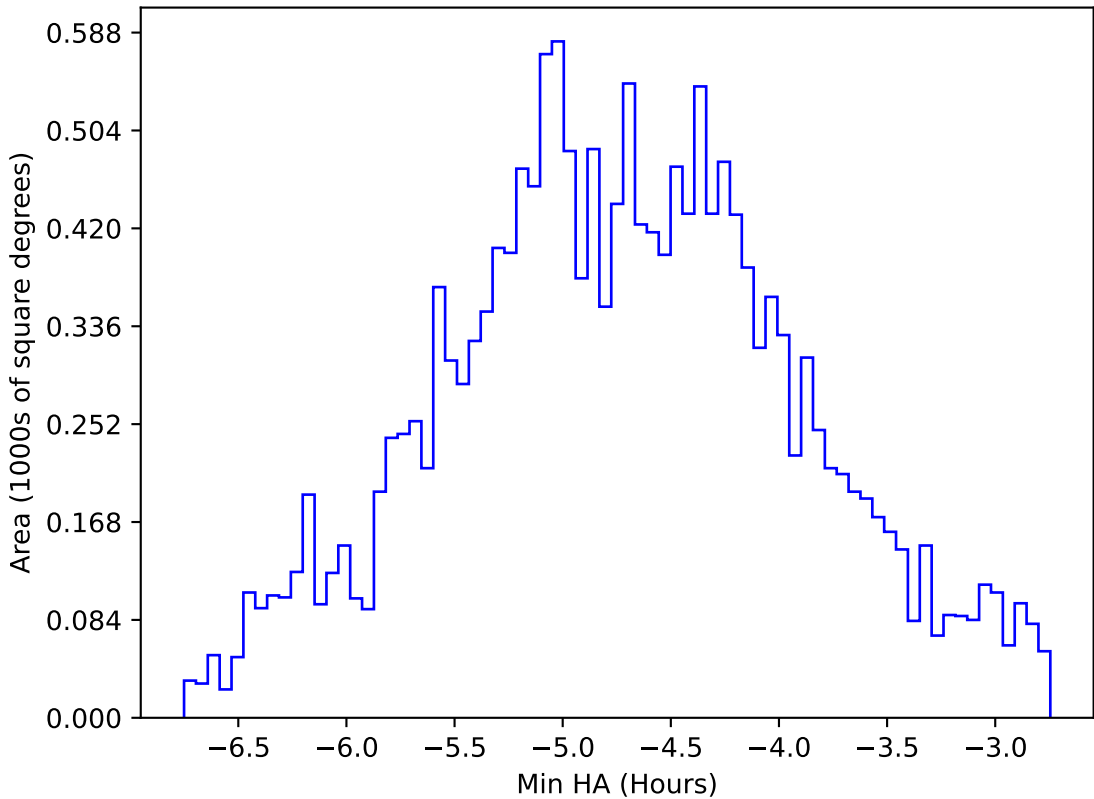
ddf_acor_sf15_lsf20_lsr20_v3.4_10yrs WFD all bands: Min HA
