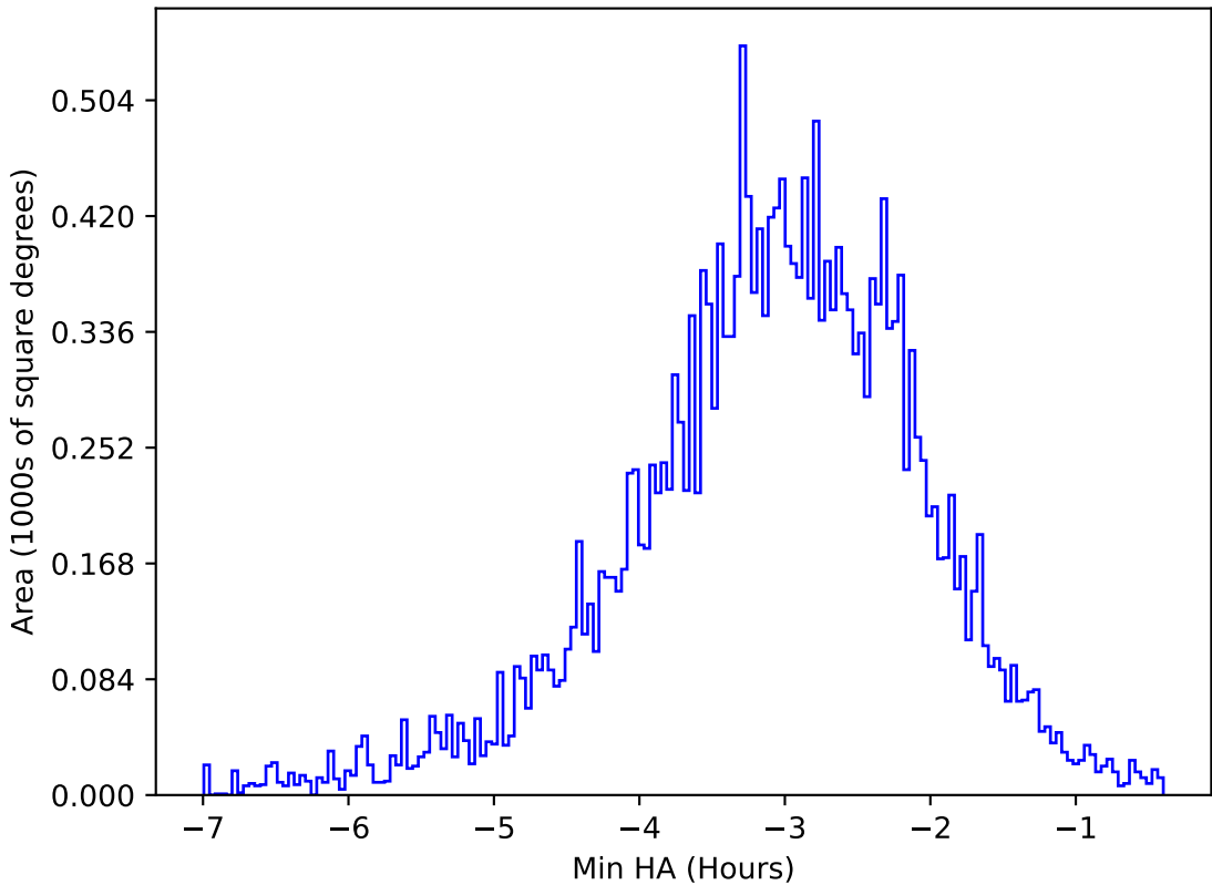
ddf_acor_sf15_lsf20_lsr20_v3.4_10yrs All sky u band: Min HA
