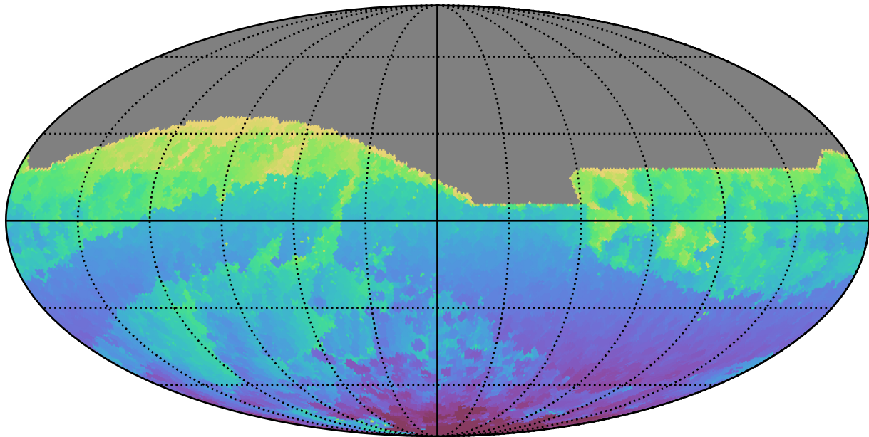
ddf_acor_sf15_lsf20_lsr20_v3.4_10yrs All sky r band: Min HA
