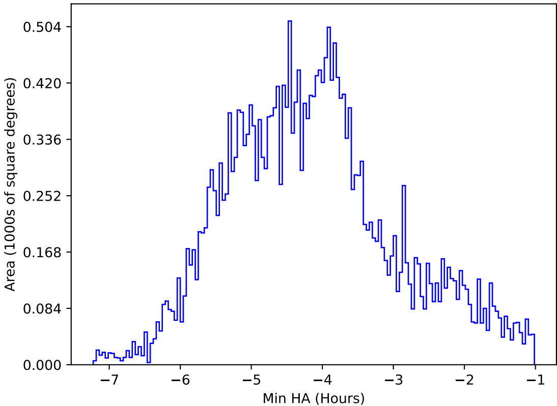
ddf_acor_sf15_ls20_lsr20_v3.4_10yrs All sky r band: Min HA
