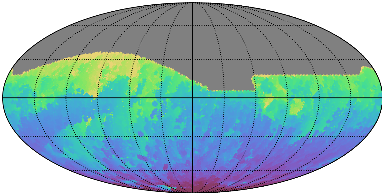
ddf_acor_sf15_lsf20_lsr20_v3.4_10yrs All sky i band: Min HA
