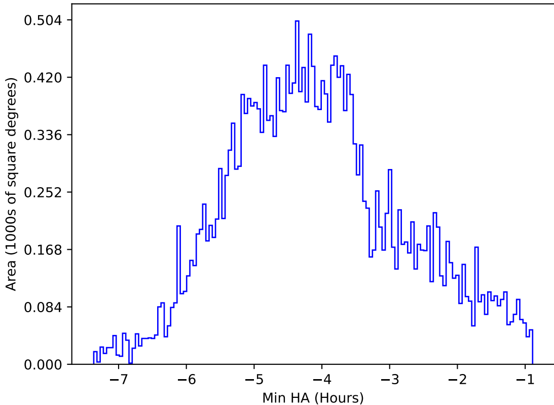
ddf_acor_sf15_ls20_lsr20_v3.4_10yrs All sky i band: Min HA
