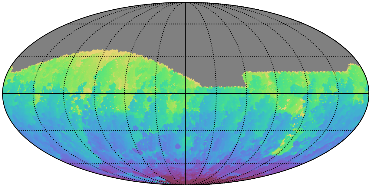
ddf_acor_sf15_lsf20_lsr20_v3.4_10yrs All sky g band: Min HA
