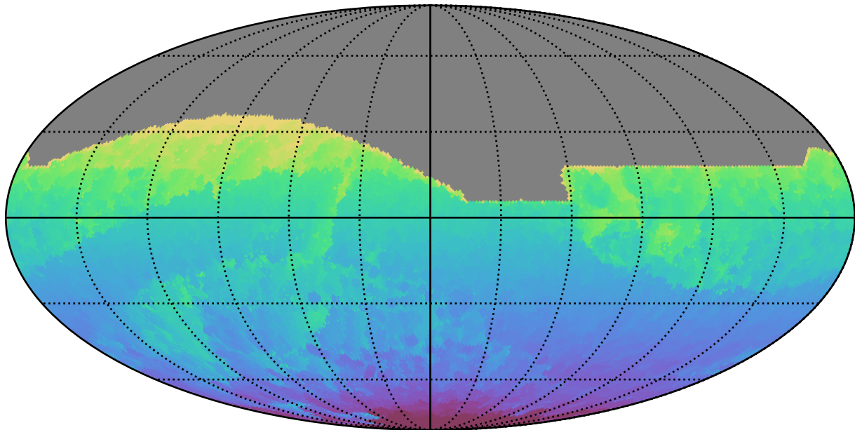
ddf_acor_sf15_lsf20_lsr20_v3.4_10yrs All sky all bands: Min HA
