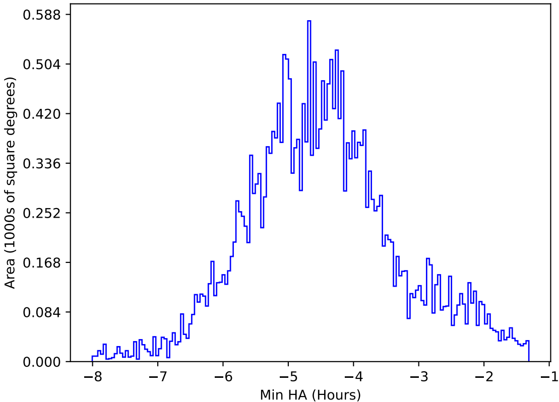
ddf_acor_sf15_lsf20_lsr20_v3.4_10yrs All sky all bands: Min HA
