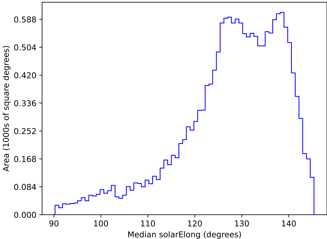
ddf_acor_sf15_lsf20_lsr20_v3.4_10yrs WFD z band: Median solarElong
