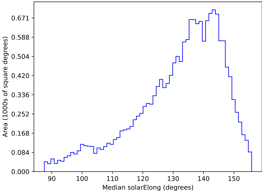
ddf_acor_sf15_lsf20_lsr20_v3.4_10yrs WFD u band: Median solarElong
