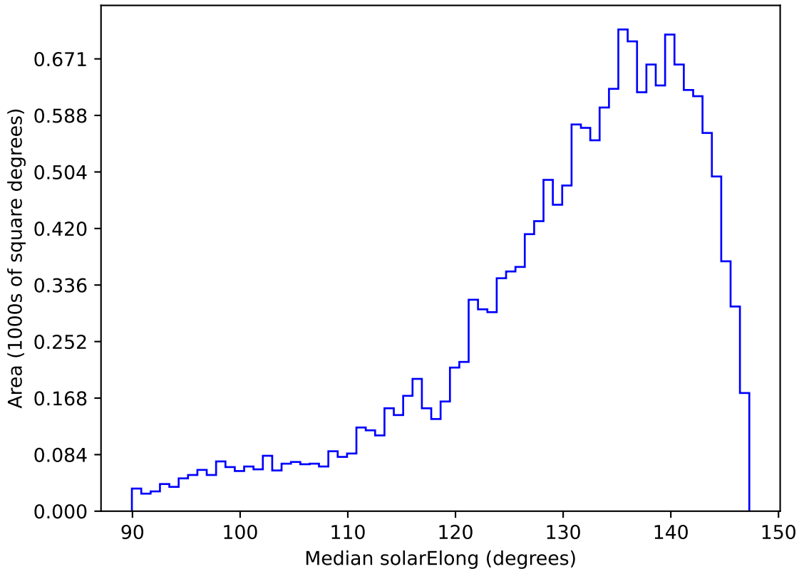
ddf_acor_sf15_lsf20_lsr20_v3.4_10yrs WFD r band: Median solarElong
