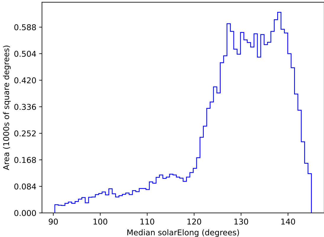
ddf_acor_sf15_lsf20_lsr20_v3.4_10yrs WFD i band: Median solarElong
