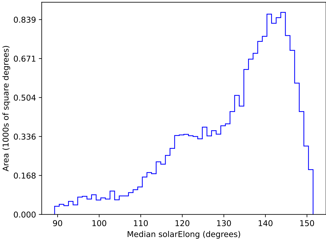
ddf_acor_sf15_lsf20_lsr20_v3.4_10yrs WFD g band: Median solarElong
