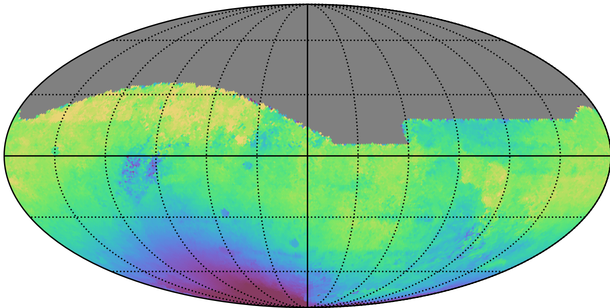
ddf_acor_sf15_lsf20_lsr20_v3.4_10yrs All sky r band: Median solarElong
