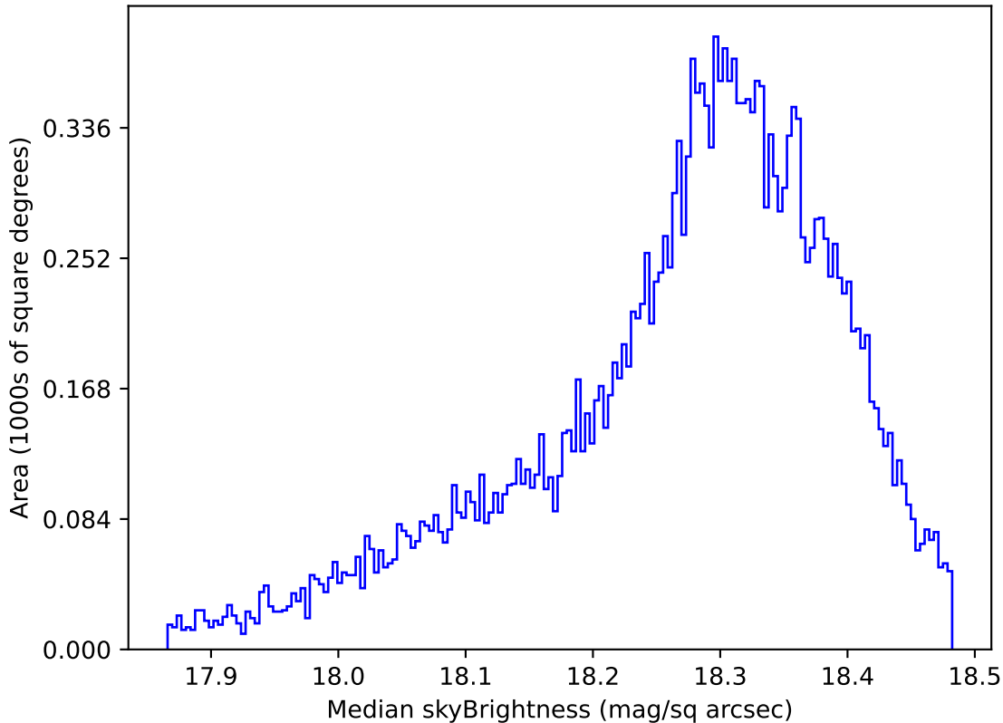
ddf_acor_sf15_lsf20_lsr20_v3.4_10yrs Yr 1 y band: Median skyBrightness
