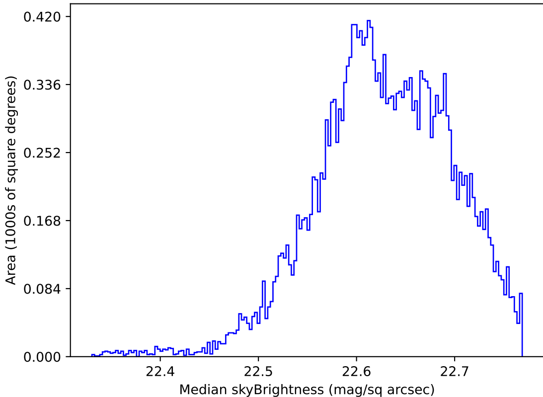
ddf_acor_sf15_lsf20_lsr20_v3.4_10yrs Yr 1 u band: Median skyBrightness
