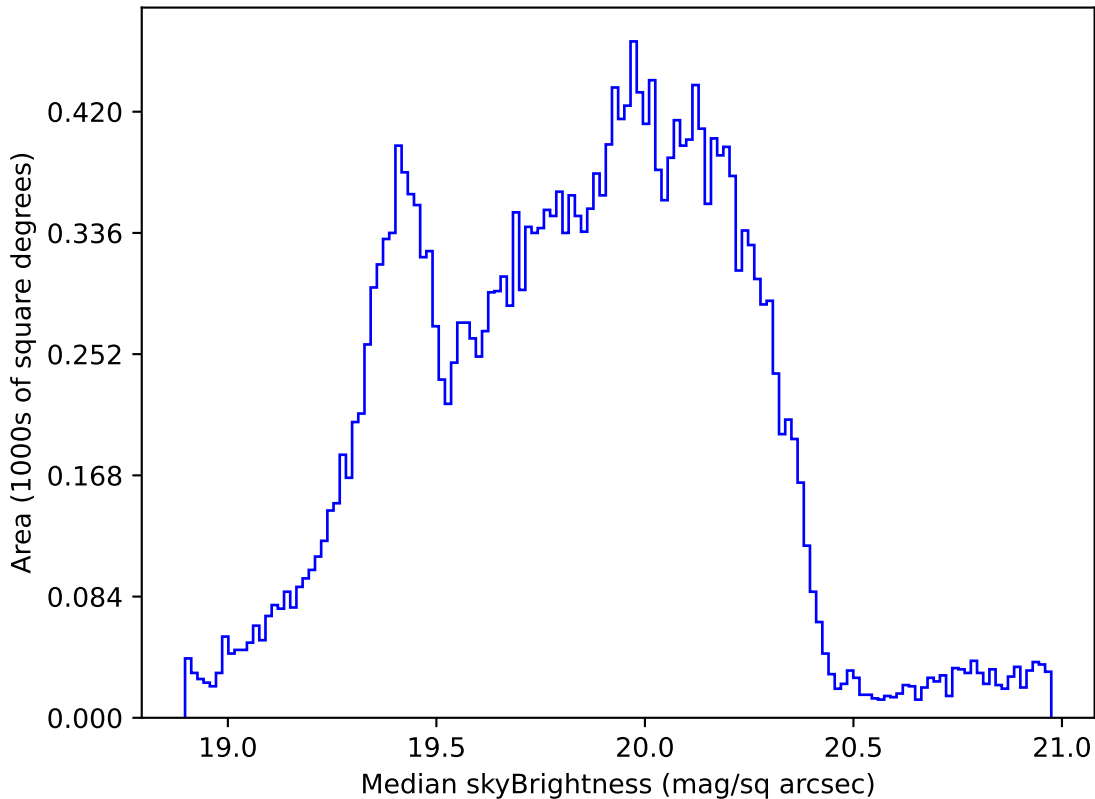
ddf_acor_sf15_lsf20_lsr20_v3.4_10yrs Yr 1 all bands: Median skyBrightness
