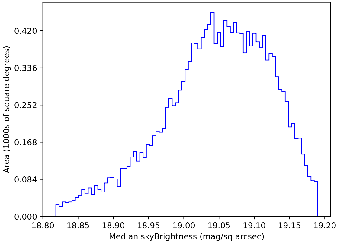
ddf_acor_sf15_lsf20_lsr20_v3.4_10yrs WFD z band: Median skyBrightness
