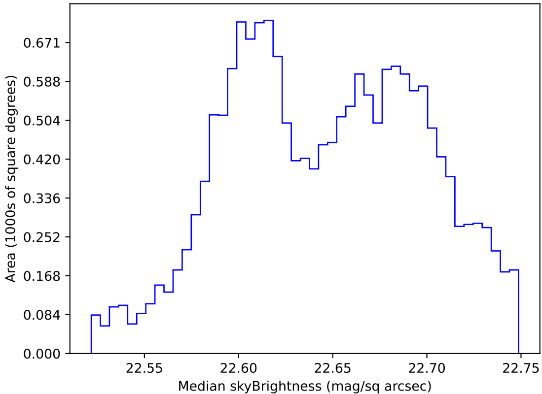
ddf_acor_sf15_lsf20_lsr20_v3.4_10yrs WFD u band: Median skyBrightness
