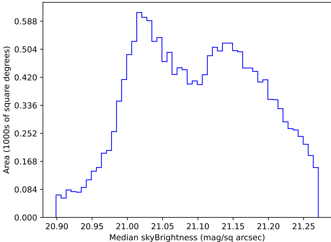
ddf_acor_sf15_lsf20_lsr20_v3.4_10yrs WFD r band: Median skyBrightness
