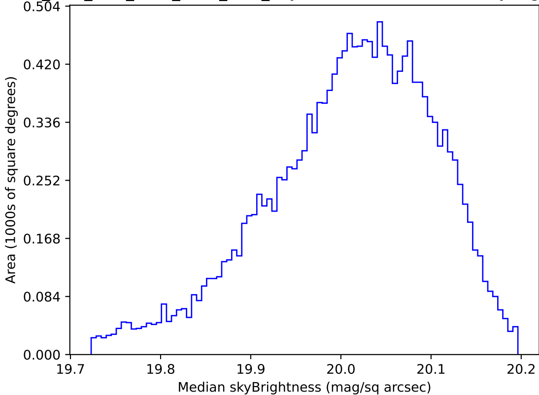
ddf_acor_sf15_lsf20_lsr20_v3.4_10yrs WFD i band: Median skyBrightness
