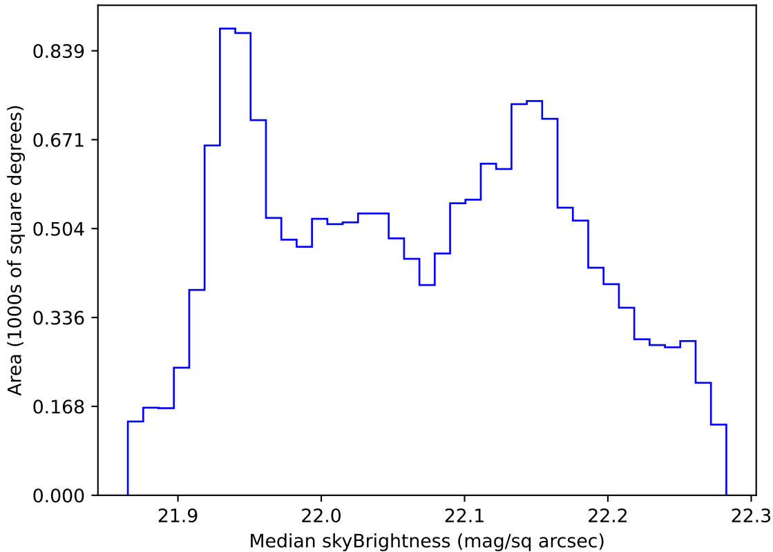
ddf_acor_sf15_lsf20_lsr20_v3.4_10yrs WFD g band: Median skyBrightness
