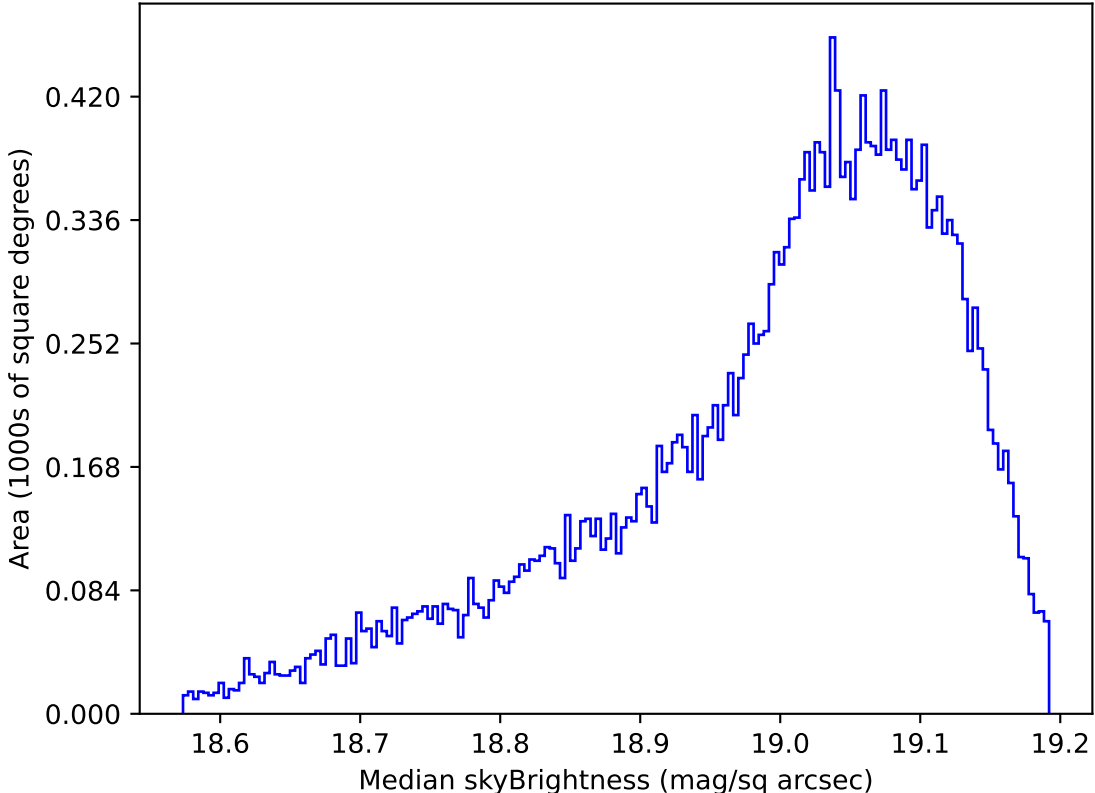
ddf_acor_sf15_lsf20_lsr20_v3.4_10yrs All sky z band: Median skyBrightness
