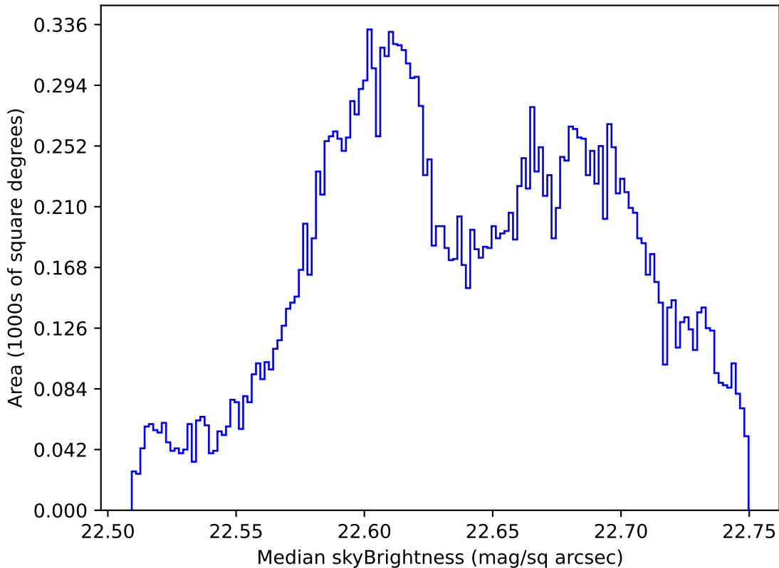
ddf_acor_sf15_lsf20_lsr20_v3.4_10yrs All sky u band: Median skyBrightness
