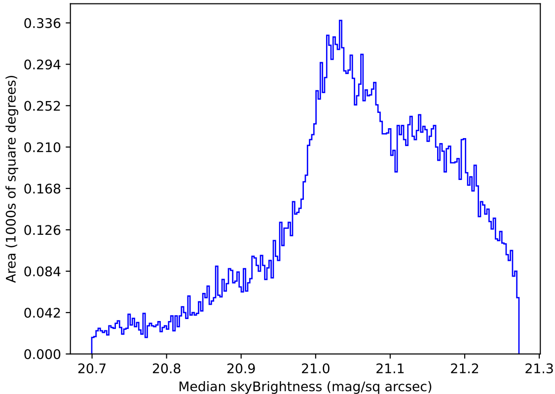
ddf_acor_sf15_lsf20_lsr20_v3.4_10yrs All sky r band: Median skyBrightness
