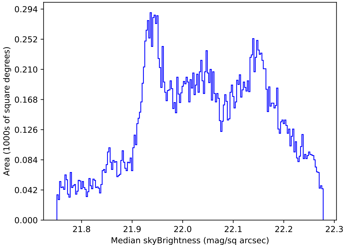
ddf_acor_sf15_lsf20_lsr20_v3.4_10yrs All sky g band: Median skyBrightness
