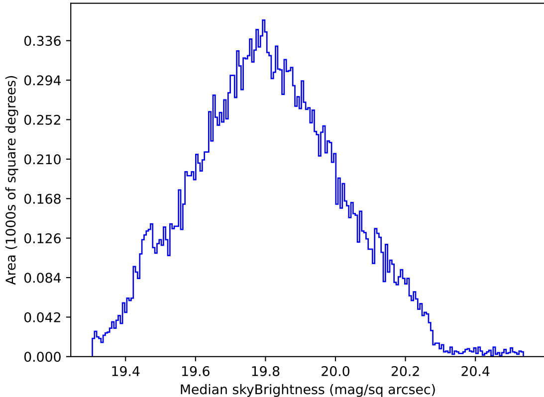
ddf_acor_sf15_lsf20_lsr20_v3.4_10yrs All sky all bands: Median skyBrightness
