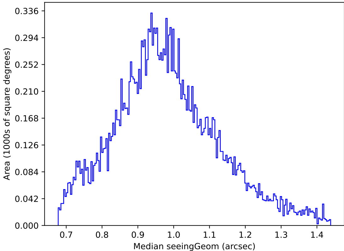
ddf_acor_sf15_lsf20_lsr20_v3.4_10yrs Yr 1 u band: Median seeingGeom
