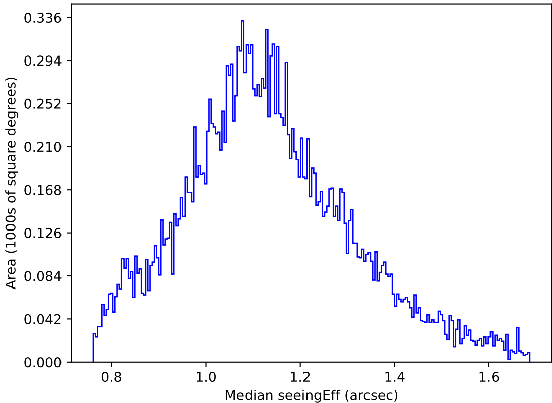
ddf_acor_sf15_lsf20_lsr20_v3.4_10yrs Yr 1 u band: Median seeingEff
