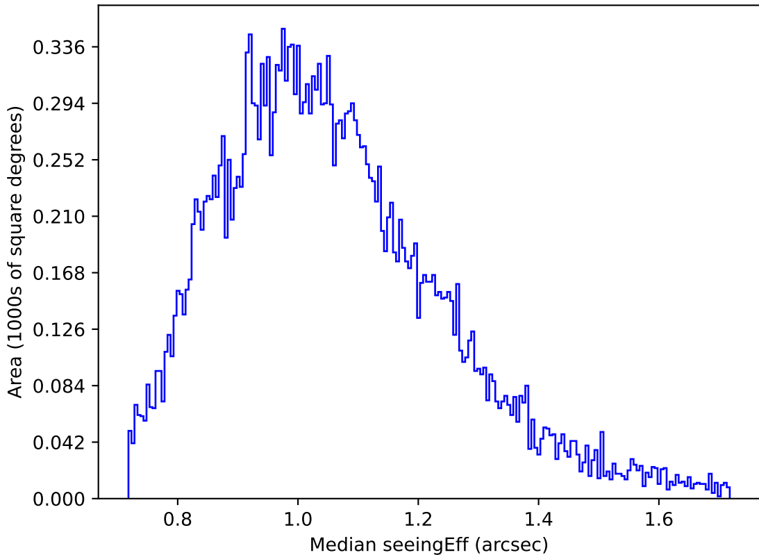
ddf_acor_sf15_lsf20_lsr20_v3.4_10yrs Yr 1 g band: Median seeingEff
