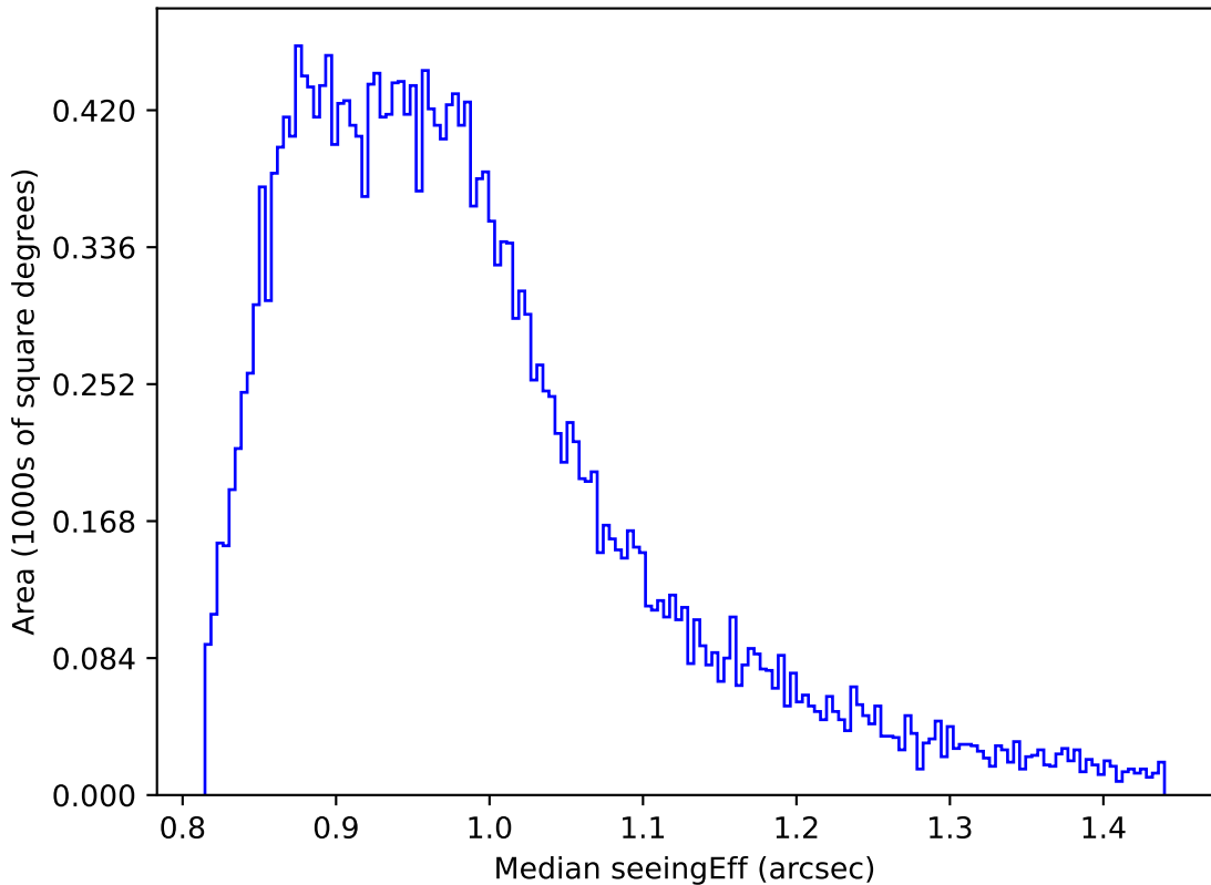
ddf_acor_sf15_lsf20_lsr20_v3.4_10yrs Yr 1 all bands: Median seeingEff
