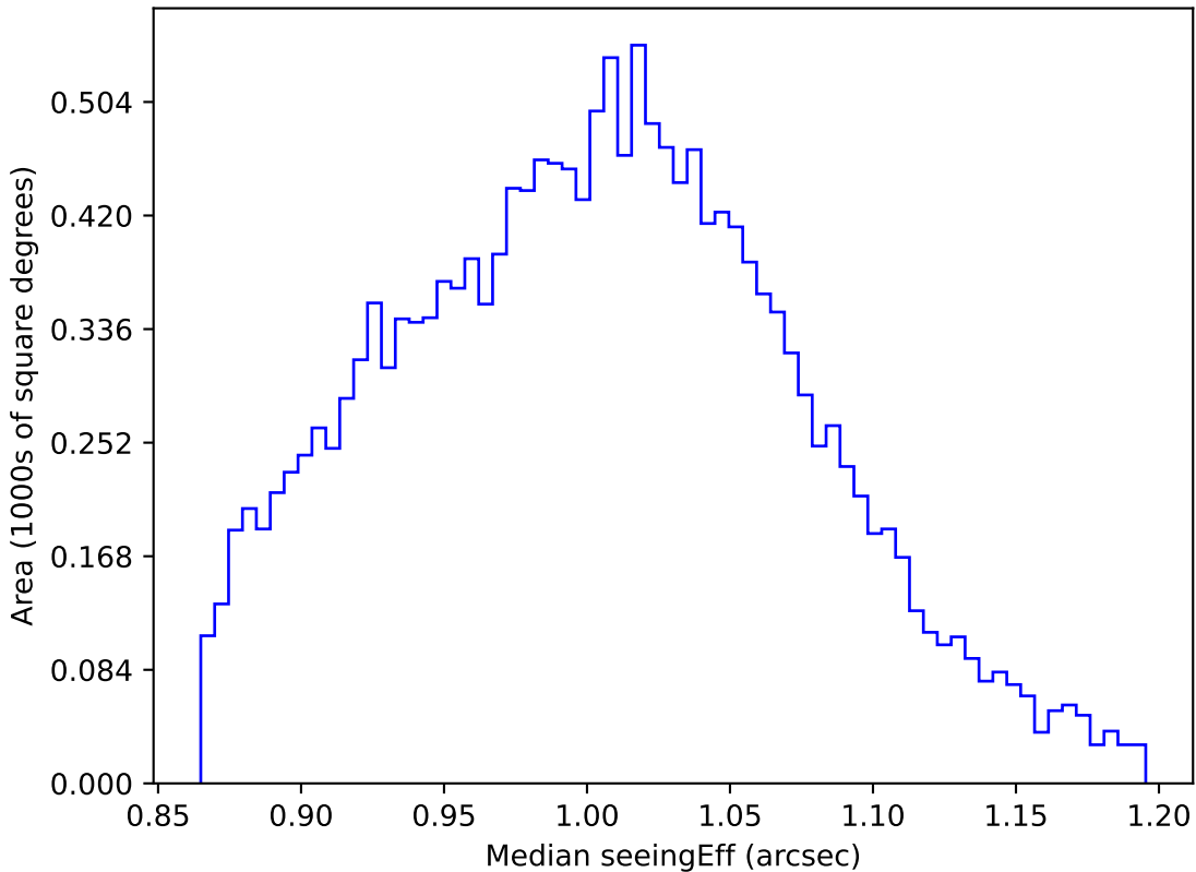
ddf_acor_sf15_lsf20_lsr20_v3.4_10yrs WFD z band: Median seeingEff
