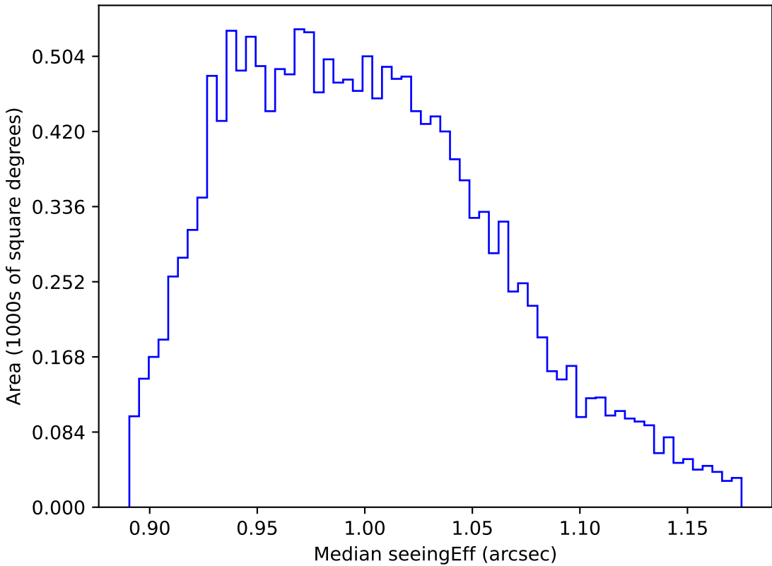
ddf_acor_sf15_lsf20_lsr20_v3.4_10yrs WFD y band: Median seeingEff
