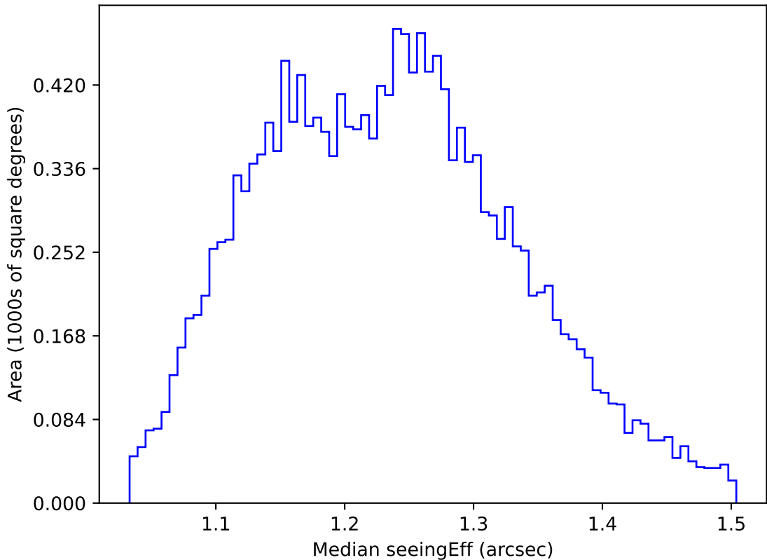
ddf_acor_sf15_lsf20_lsr20_v3.4_10yrs WFD u band: Median seeingEff
