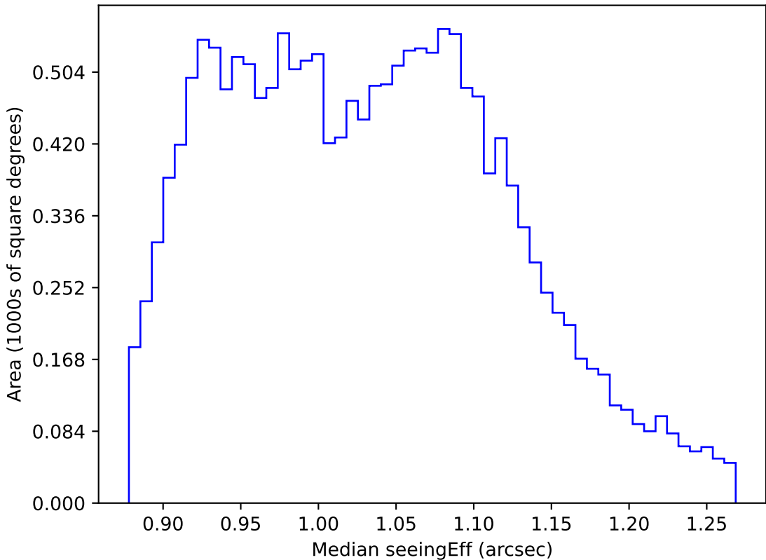
ddf_acor_sf15_lsf20_lsr20_v3.4_10yrs WFD r band: Median seeingEff
