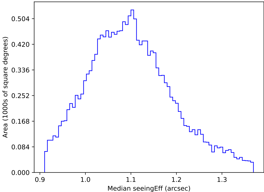
ddf_acor_sf15_lsf20_lsr20_v3.4_10yrs WFD g band: Median seeingEff
