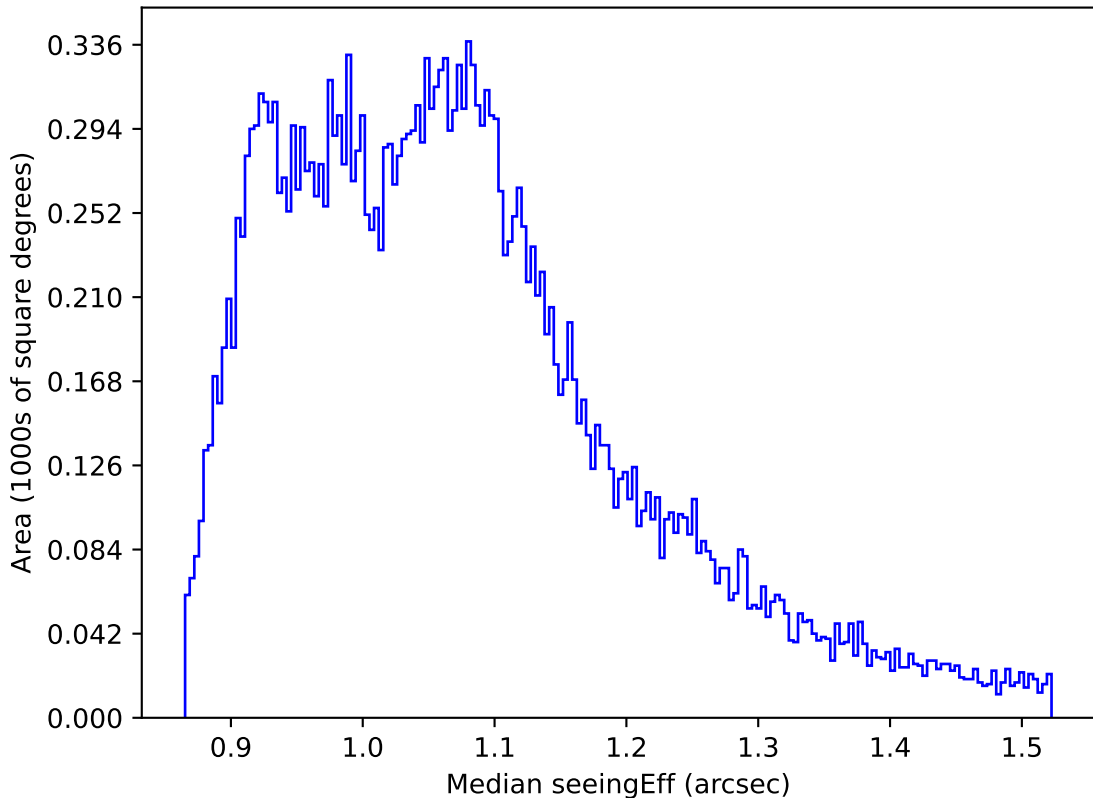
ddf_acor_sf15_lsf20_lsr20_v3.4_10yrs All sky r band: Median seeingEff
