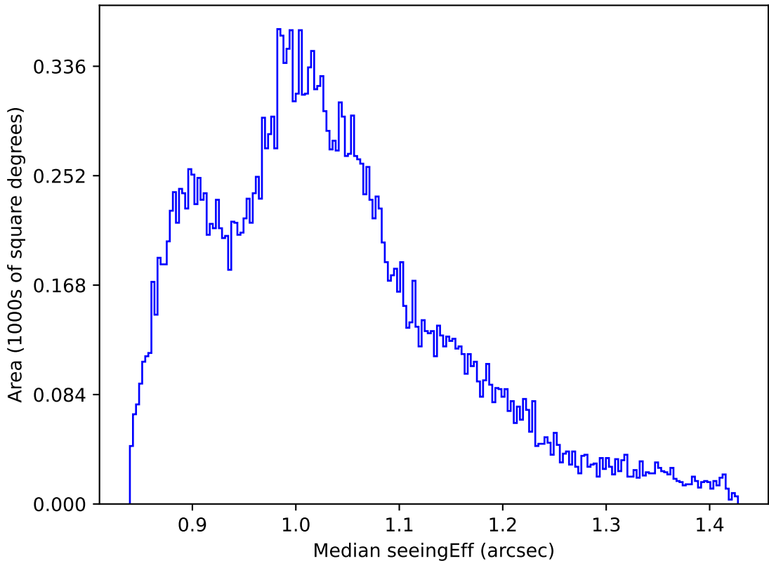
ddf_acor_sf15_lsf20_lsr20_v3.4_10yrs All sky i band: Median seeingEff
